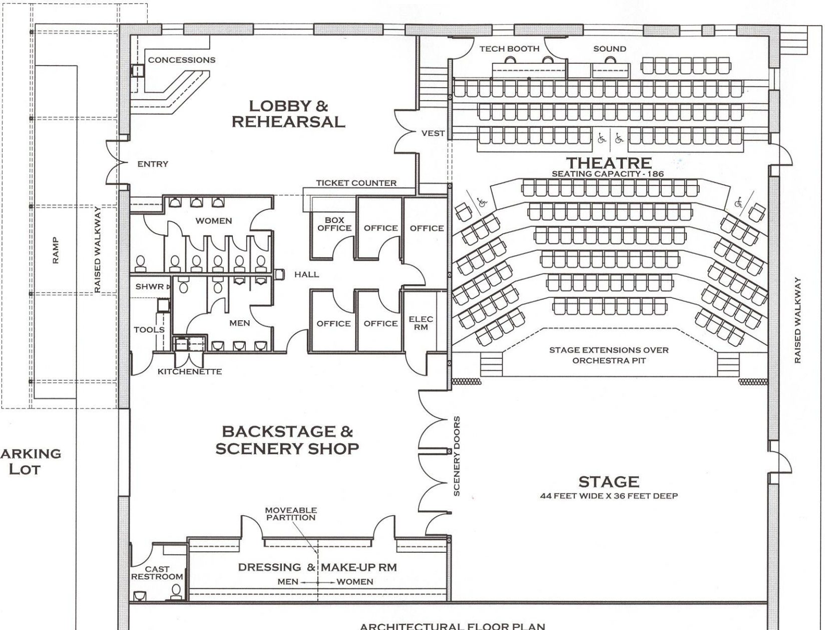
ARCHITECTURAL FLOOR PLAN
